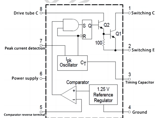
logic diagram
