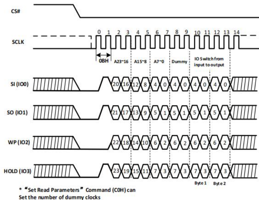
Figure-16. Read Data Bytes at Higher Speed Sequence Diagram (QPI)
