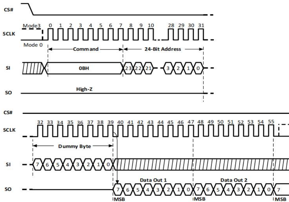
Figure-15. Read Data Bytes at Higher Speed Sequence Diagram
