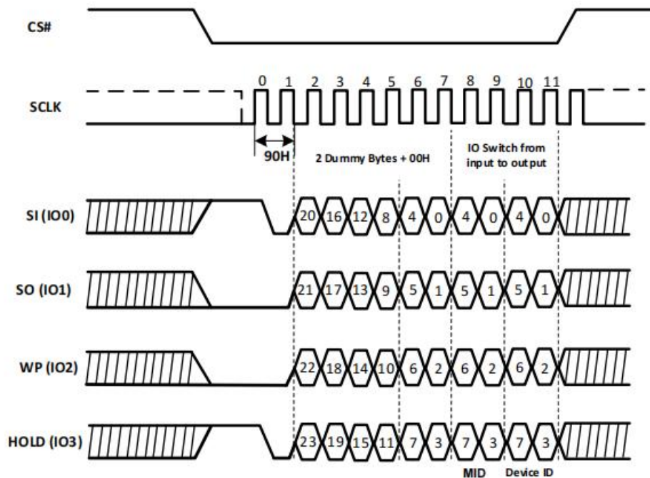
Figure-64. Read Electronic Manufacturer ID & Device ID Sequence Diagram (QPI)
