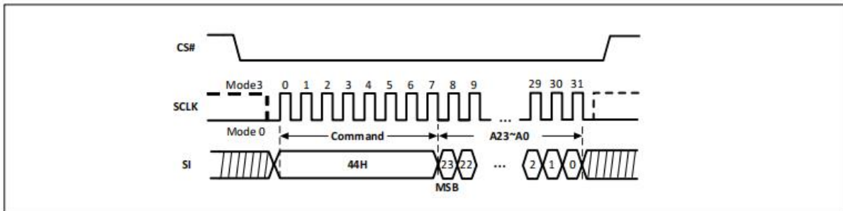
Figure-46. Erase Security Register Sequence Diagram
