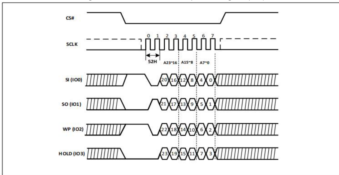
Figure-35. Half Block Erase Sequence Diagram (QPI)
