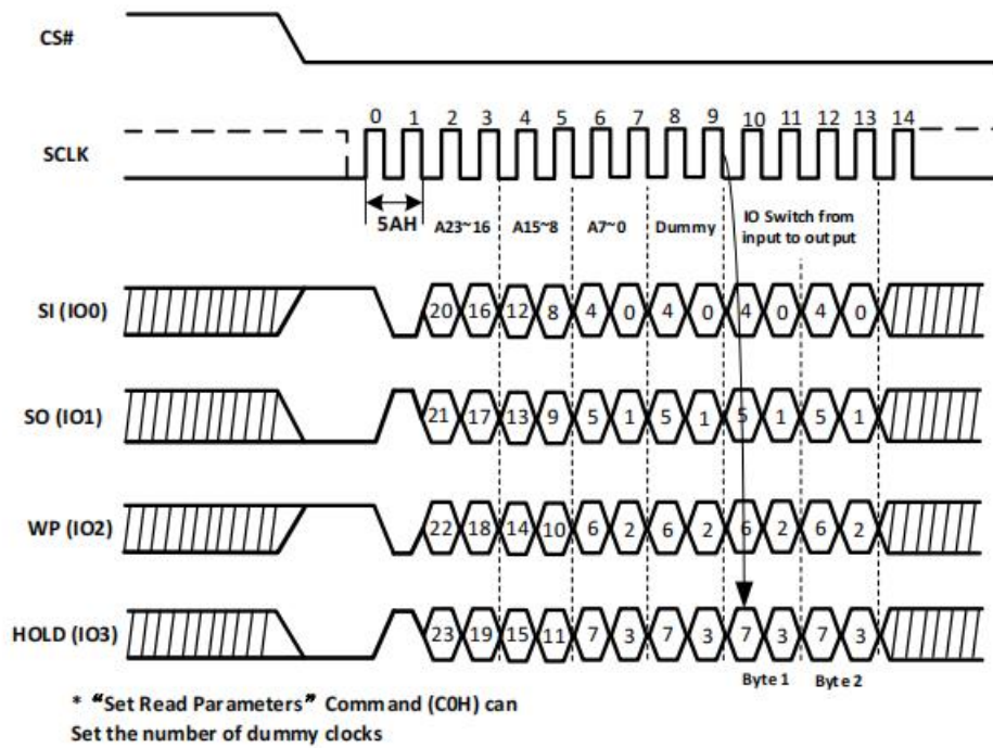
Figure-76. Read Serial Flash Discoverable Parameter Sequence Diagram (QPI)
