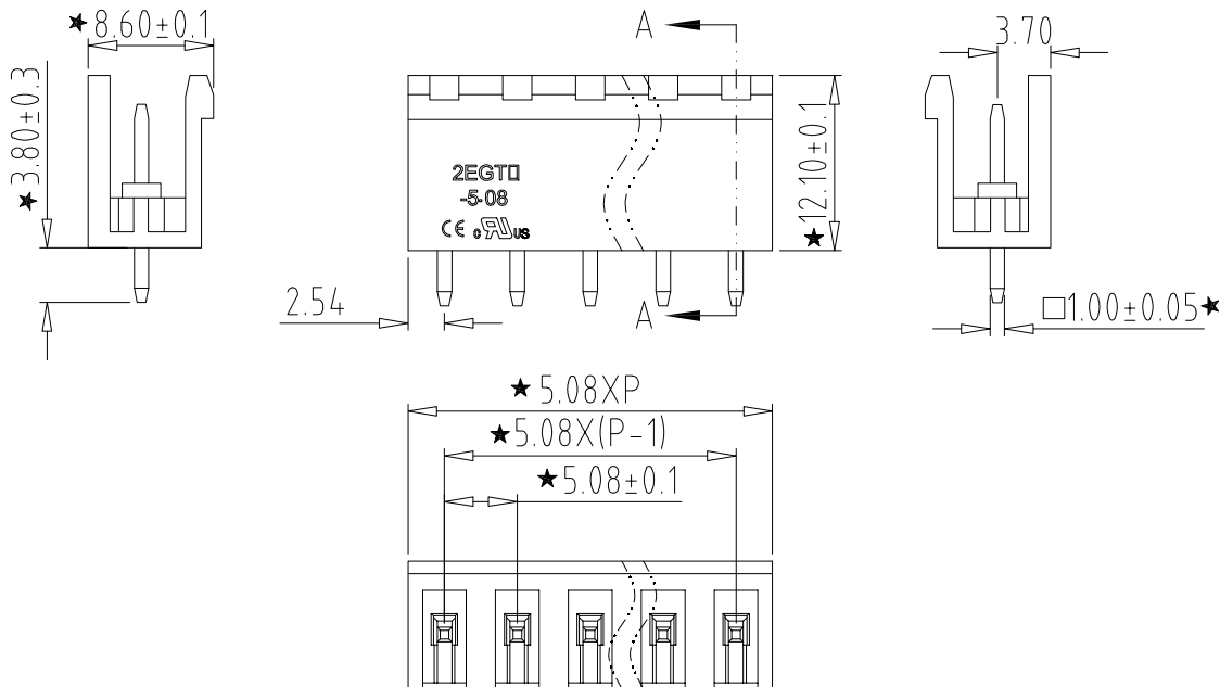
PCB Layout
