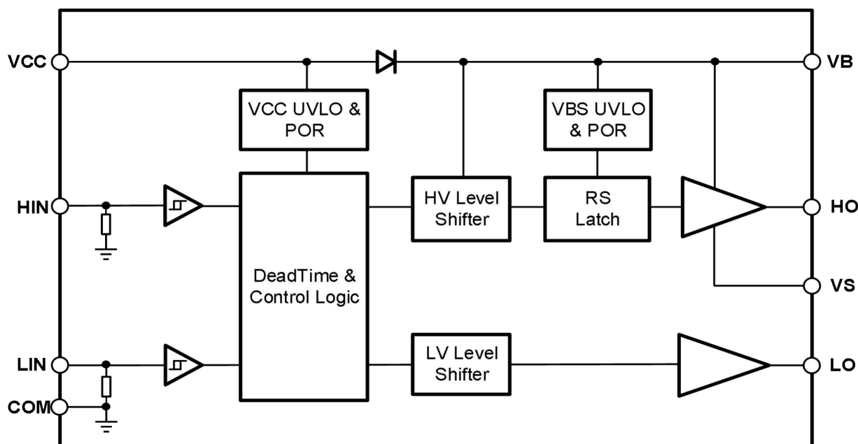
Figure10-1 Function Block Diagram of IRS2304STR
