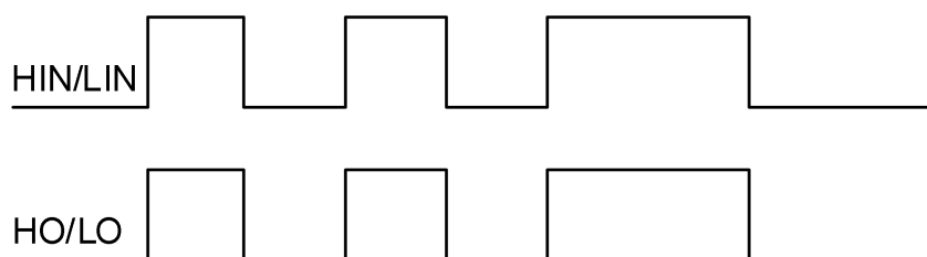
Figure 9-1 IRS2186STR Input and output timing waveform
