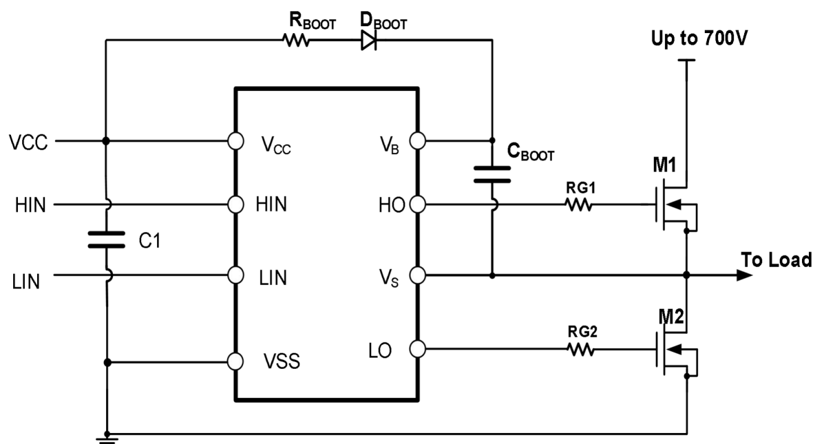
Figure10-2 Typical application circuit of IRS2186STR
