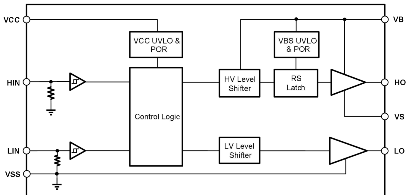
Figure 10-1 Function Block Diagram of IRS2186STR
