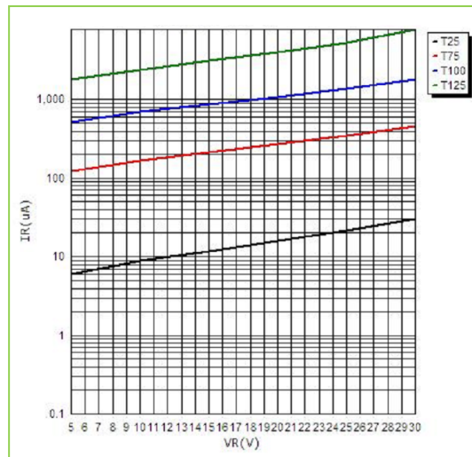
Reverse current( I_R ) vs Reverse voltage( V_R )
