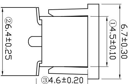
DIMENSION TABLE:
