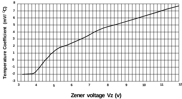
Temperature Coefficient
