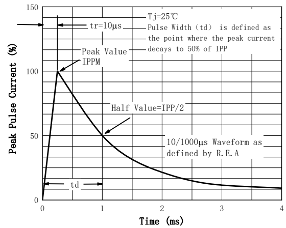
FIG.2 Pulse Waveform
