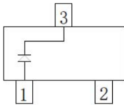
BAS70Q Marking:73
