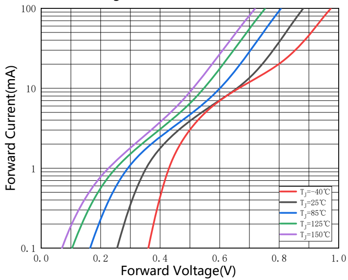
Fig.3: Forward Characteristics
