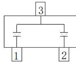
BAS70-06Q Marking:76
