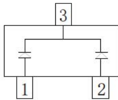
BAS70-05Q Marking:75
