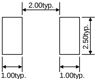
Recommended Pad Layout (mm)
