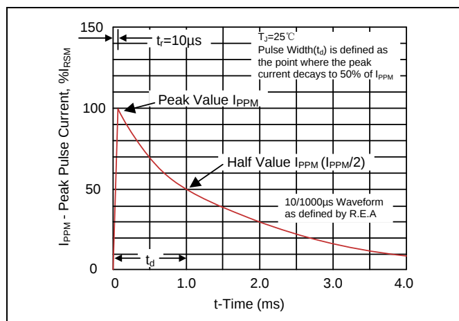
Figure 2. 10/1000μs Pulse Waveforms
