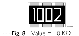
Fig. 8 Value = 10 K \Omega
