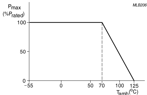
Fig. 10-2 Maximum dissipation (P) in percentage of rated power as a function of the operating ambient temperature (Tamb)
