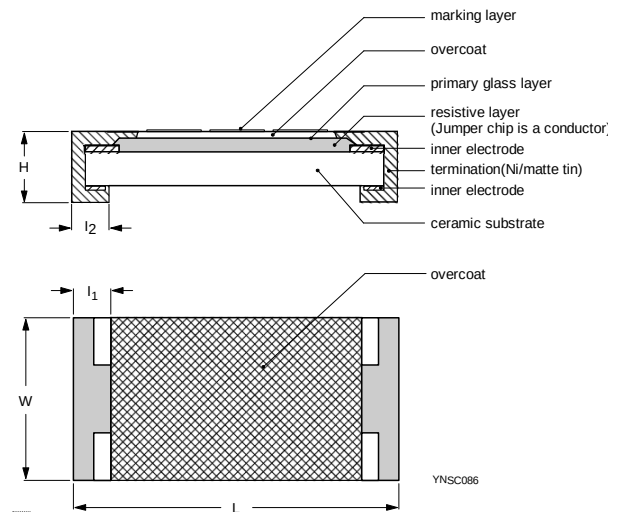
Fig. 8 Chip resistor outlines
