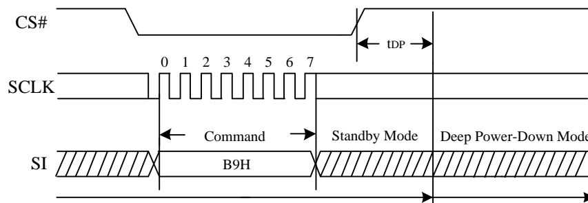
Figure 28. Deep Power-Down Sequence Diagram
