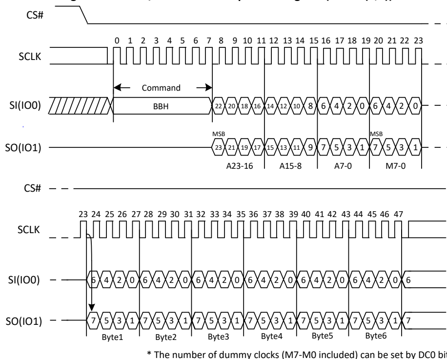
Figure 10. Dual I/O Fast Read Sequence Diagram (M5-4=(1,0))
