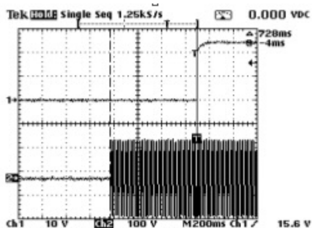
ECM100US24 start up 115 VAC at 100% load
