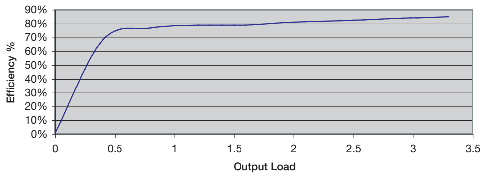
Efficiency shown for ECM100US24
