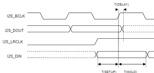
Fig. 7.2: I2S slave timing
