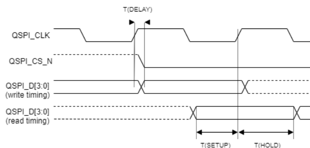
Fig. 7.1: QSPI Timing
