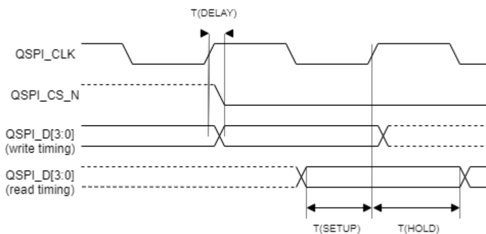
Fig. 8.1: QSPI Timing
