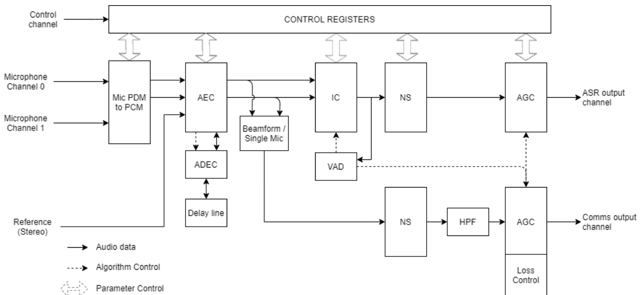
Fig. 3.1: The XVF3610 audio processing pipeline
