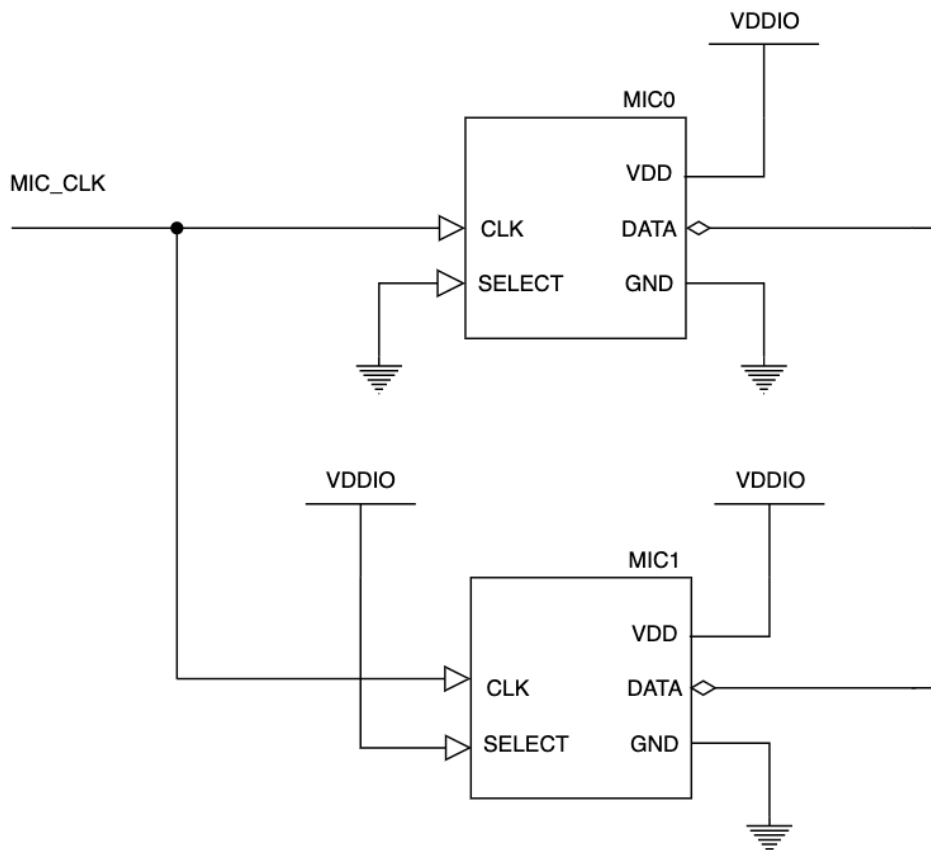
Fig. 5.1: PDM microphone schematic
