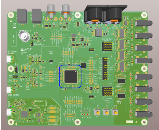
Figure 2: xcore.ai device
