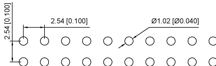
PCB LAYOUT
