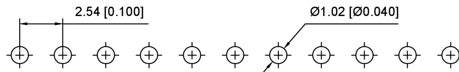
PCB LAYOUT
