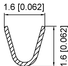
SECTION:A-A SCALE:1:1
