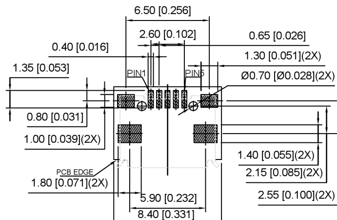
RECOMMENDED PCB LAYOUT(TOP VIEW) DEFAULT TOLERANCE: ±0.05
