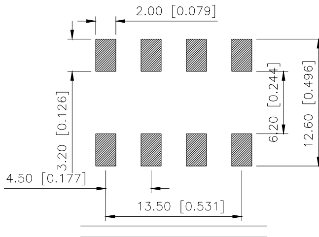
PCB LAYOUT
