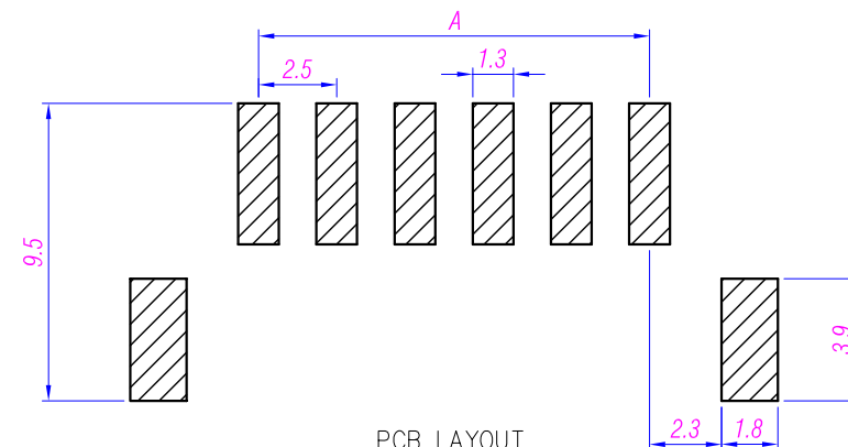
PCB LAYOUT
