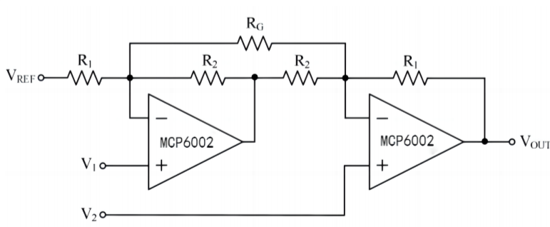
Figure 15 Instrumentation Amplifier
