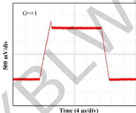
Figure 6 Large-Signal Step Response at 2.7V
