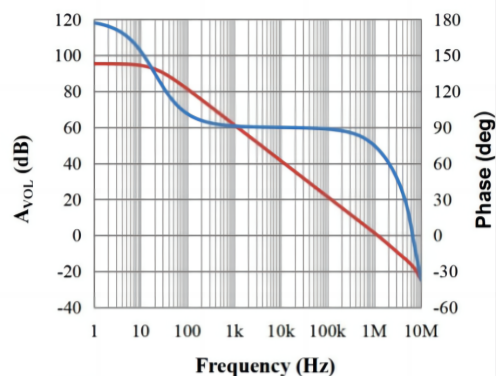
Figure 2 Open-loop Gain and Phase as function of Frequency
