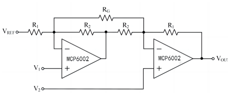
Figure 15 Instrumentation Amplifier
