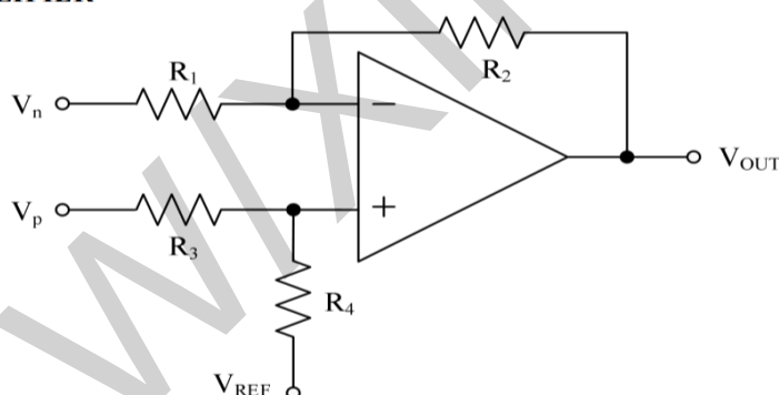
Figure 14 Differential Amplifier
