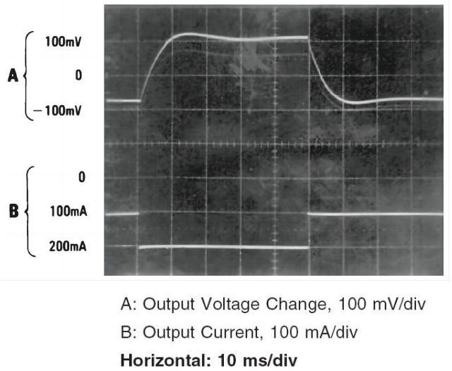
FIGURE 25. Load Transient Response of Flyback Regulator of Figure 21, -15V Output
