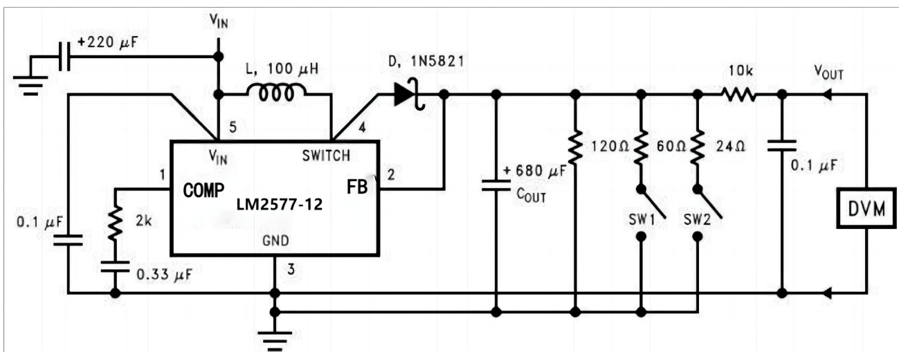
Figure.1 Circuit Used to Specify System Parameters for 12V Versions L = 415-0930 (AIE) D = any manufacturer COUT = Sprague Type 673D Electrolytic 680μF, 20V
