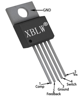
TO-220-5
