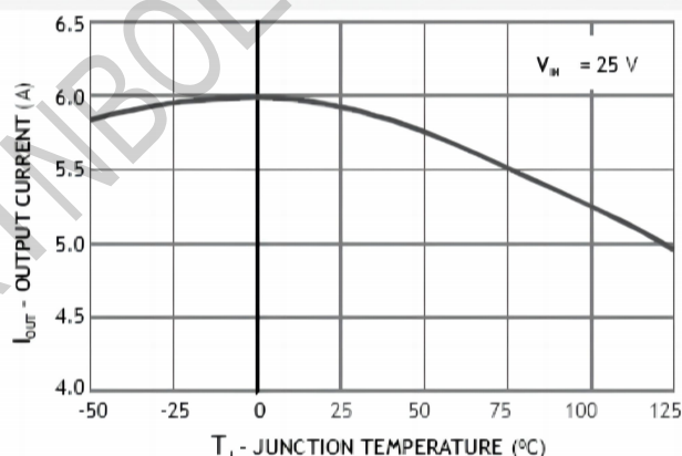
CURRENT LIMIT
