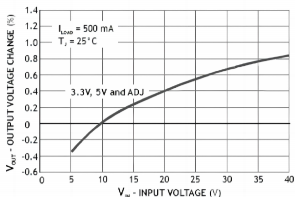
LINE REGULATION
