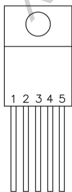
TO220-5
