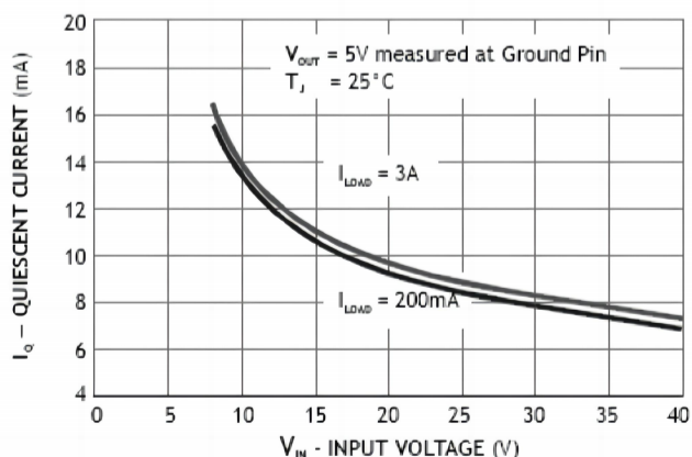
QUIESCENT CURRENT
