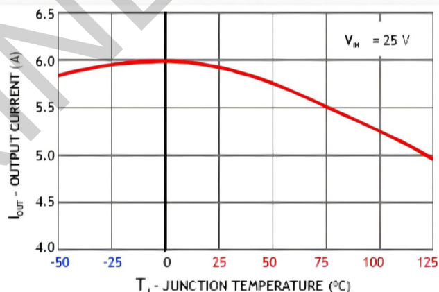
CURRENT LIMIT
