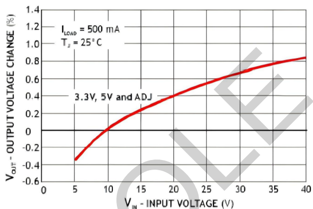
LINE REGULATION
