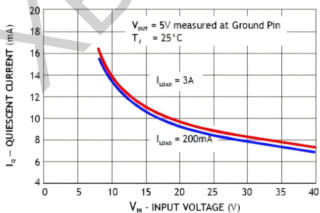
QUIESCENT CURRENT
