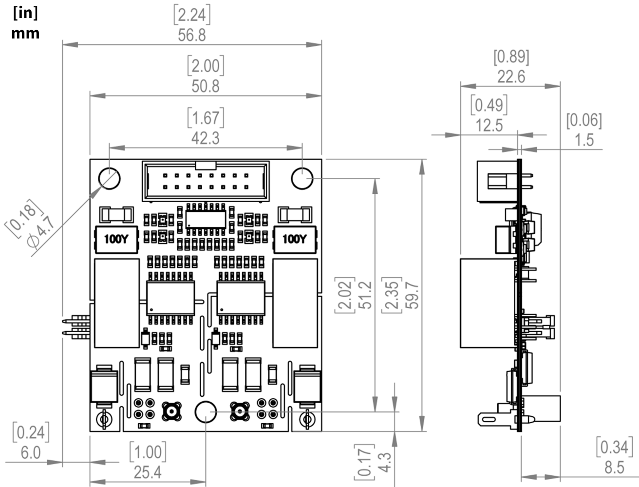
Figure 29: Dimensions of the CGD1700HB2M-UNA gate driver
