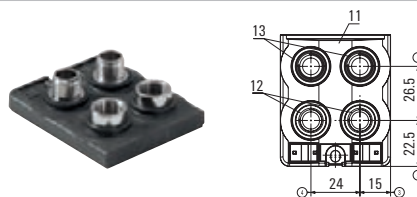
I/O cover (4M12 | 3 pin, 1 socket)
