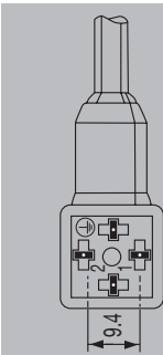
Contact gap 9.4 mm Industry standard Type: VSC
