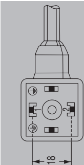
Contact gap 18 mm Type: VSA
