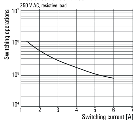
Electrical endurance
