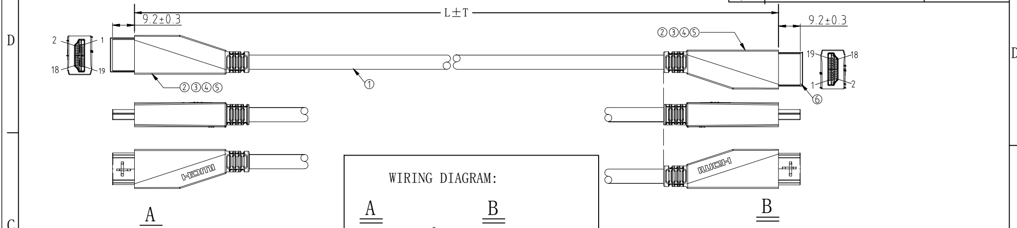
WIRE DIAGRAM
