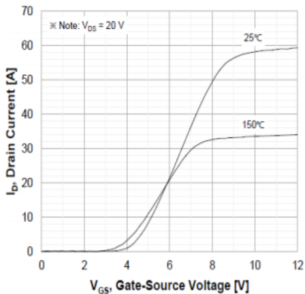
Transfer characteristics
