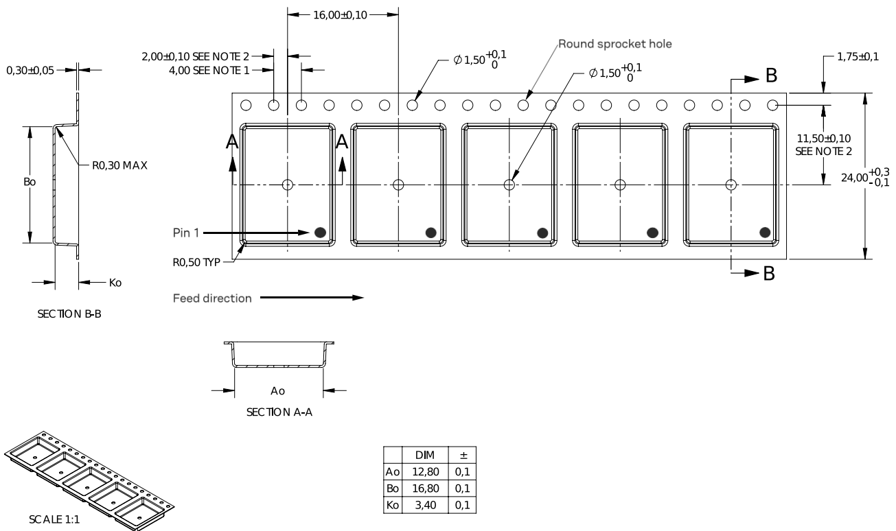
Figure 5: Dimensions (in mm) and orientation for NEO-M8L-06B modules on tape
