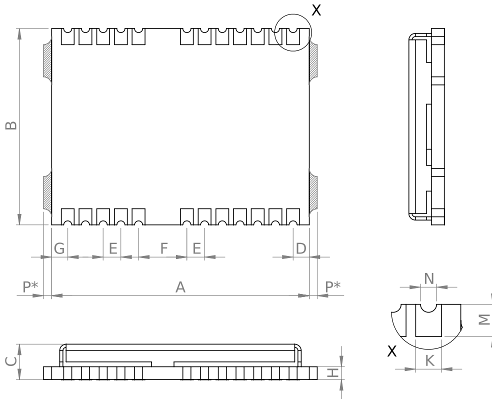
Figure 4: NEO-M8L-06B mechanical drawing
