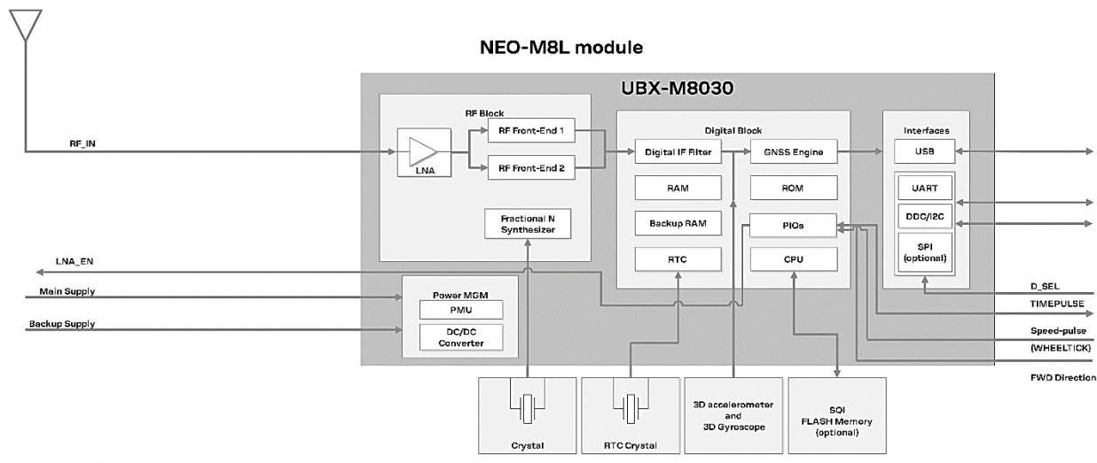
Figure 1: NEO-M8L-06B block diagram
