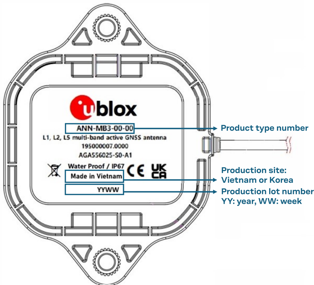
Figure 7: ANN-MB3 triple-band GNSS antenna product label.
