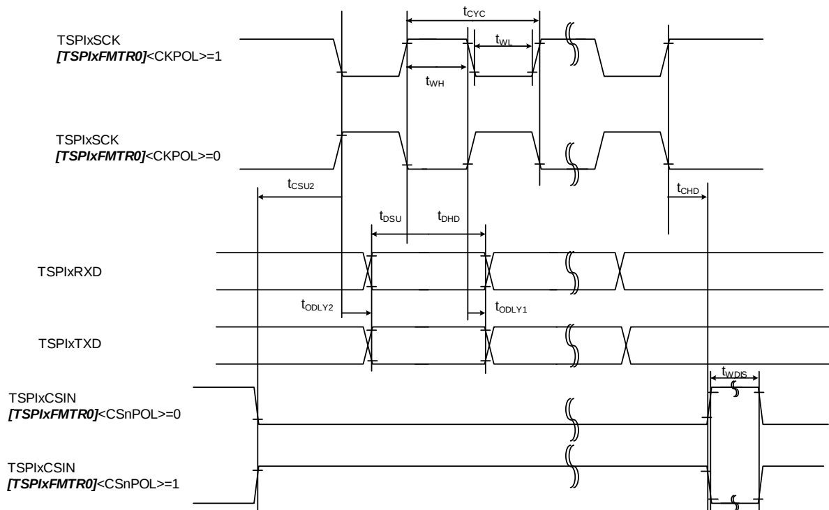
Figure 7.6 2nd clock edge sampling (Slave)
