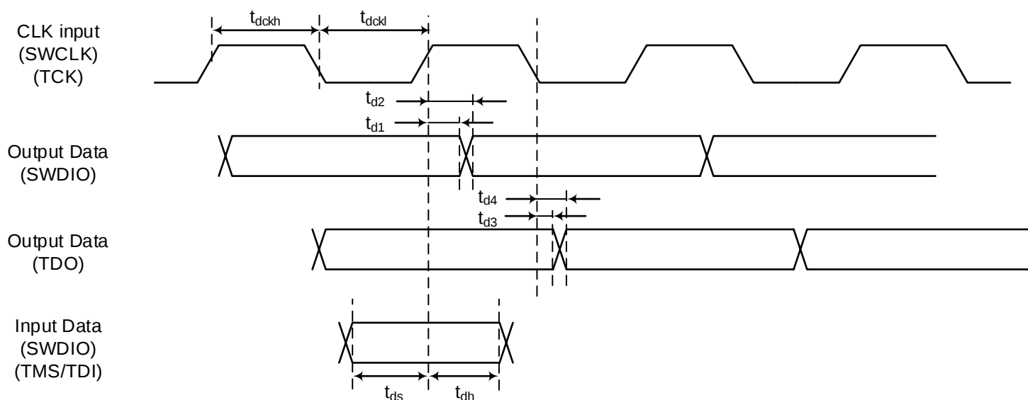
Figure 7.10 JTAG/SW waveform
