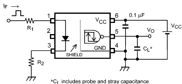
Fig. 13.1.5 Switching Time Test Circuit and Waveform
