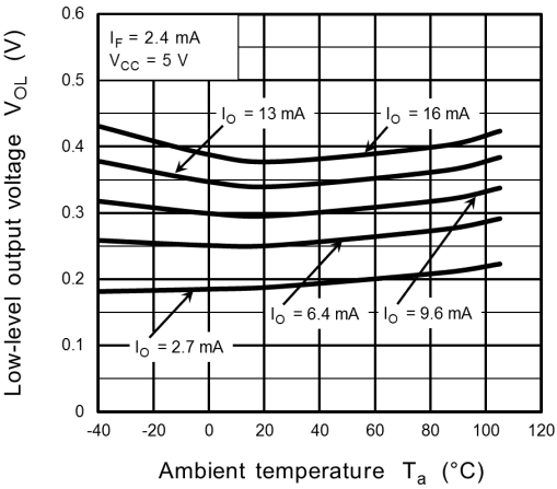
Fig. 12.2.4 V_{OL} - T_a
