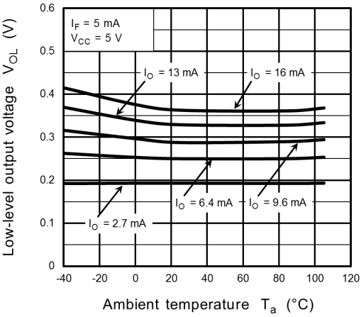
Fig. 12.2.6 V_{OL} - T_a
