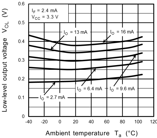
Fig. 12.2.3 V_{OL} - T_a
