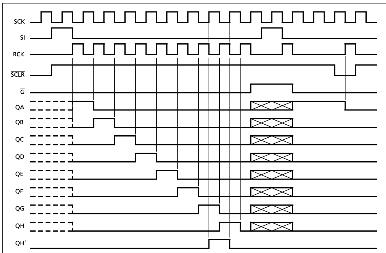
TIMING CHART
