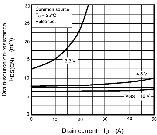
Fig. 7.5 R_{DS(ON)} - I_D
