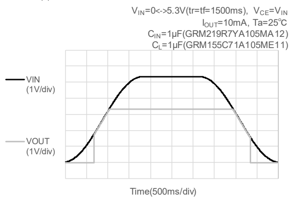
(16-2) V_{OUT(T)}=3.3V
