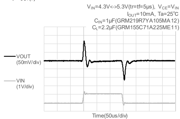
(17-2) V_{OUT(T)}=3.3V
