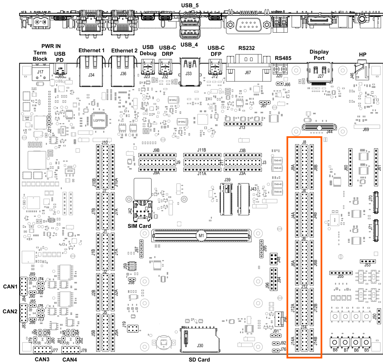
Figure 9: Aquila Development Board connectors and controls
