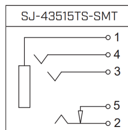
Figure 5: Audio Jack Pinout
