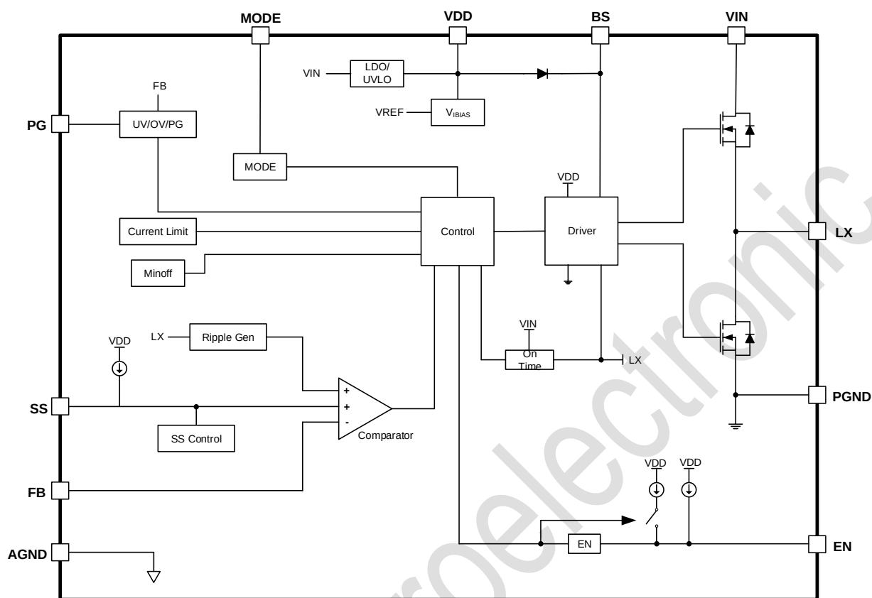
Figure 2. TMI32120 Block Diagram
