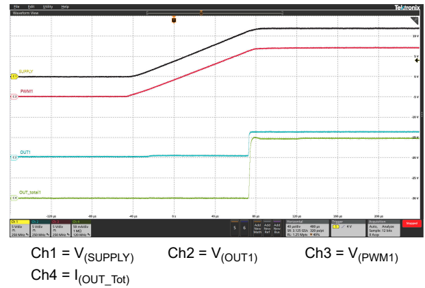
Figure 6-10. Power-Up Sequence
